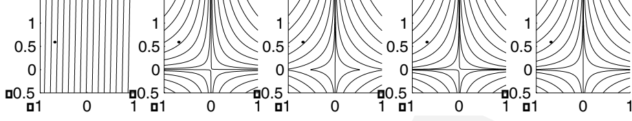
Fig. 1. PCA with kernel (11, degrees d = 1, \dots, 5 . 100 points ((x_i)_1, (x_i)_2) were generated from (x_i)_2 = (x_i)_1^2 + \text{noise} (Gaussian, with standard deviation 0.2); all (x_i)_j were rescaled according to (x_i)_j \mapsto \text{sgn}((x_i)_j) \cdot |(x_i)_j|^{1/d} . Displayed are contour lines of constant value of the first principal component. Nonlinear kernels ( d > 1 ) extract features which nicely increase along the direction of main variance in the data; linear PCA ( d = 1 ) does its best in that respect, too, but it is limited to straight directions.
