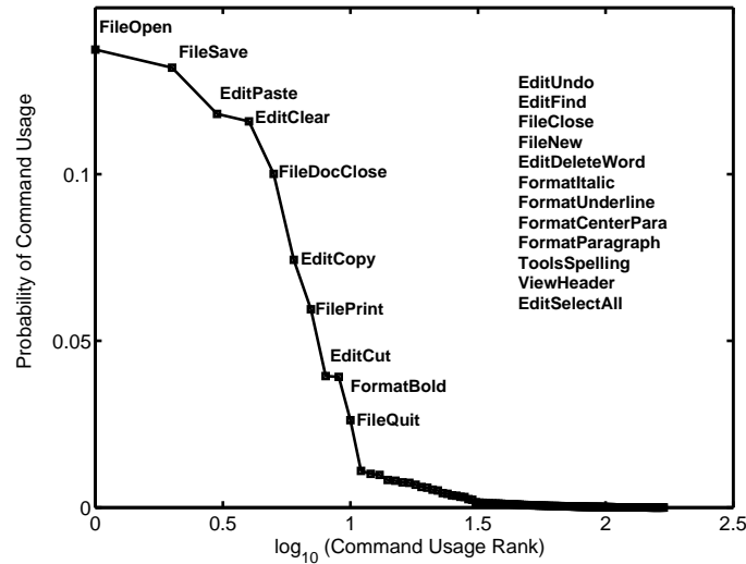
Fig. 1. The ranked normalized frequency of usage of the 169 available wordprocessor commands. Each of the ten most frequently used commands is listed at the relevant rank-point on the graph, with the remaining twelve most frequently issued commands being listed in the chart body.
