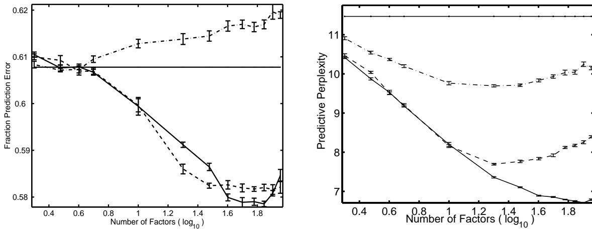
Fig. 2. The left hand plot shows the percentage of incorrect predictions against the number of model factors and the right hand plot charts the predictive perplexity of each model against model order for the PHONE dataset. The global first-order Markov chain is represented by a solid straight line, the dashed line represents the MAP estimated simplicial model, the solid line represents the VB estimated simplicial model and the dash-dot line represents the mixture model. The error bars represent one standard error.
