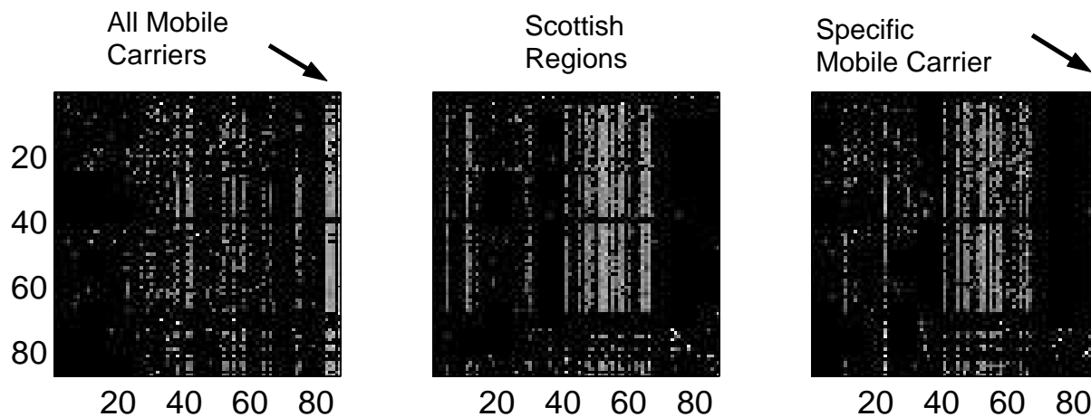
Fig. 4. The state transition matrices corresponding to factors 3, 10 & 19 for the customer under consideration.
