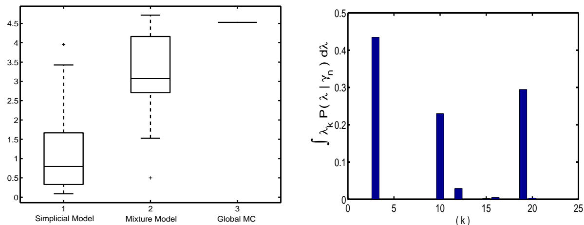
Fig. 3. The left hand plot shows the distribution of entropy rates for the transition matrices of a twenty factor mixture and simplicial mixture models (VB). The right hand plot shows the expected value of the Dirichlet variable under the variational approximation for one customer indicating the levels of participation in factor specific behaviors.
