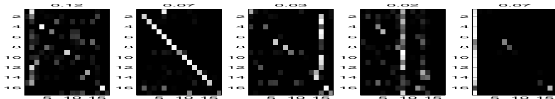
Fig. 6. State transition matrices of selected factors from a twenty-factor run produced by Simplicial Mixtures of MCs on the WEB data set.
